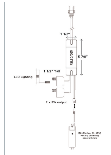
PSLED/DIM connection diagram
